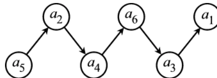
Figure 2: PROMETHEE II complete ranking
