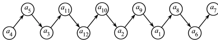
Figure 5: PROMETHEE II
